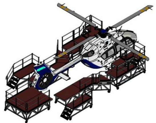
Complete dock existing of separate mobile modules
