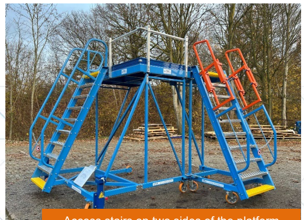
Access stairs on two sides of the platform
