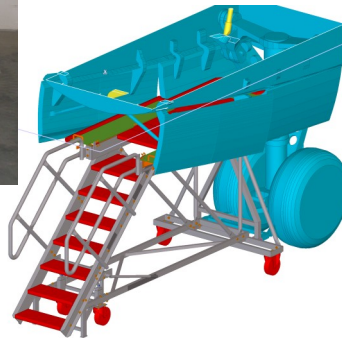
Detailed 3D scanning resulted in 3D drawing and from there to the development of the B787 Nose Landing Gear Stand.
